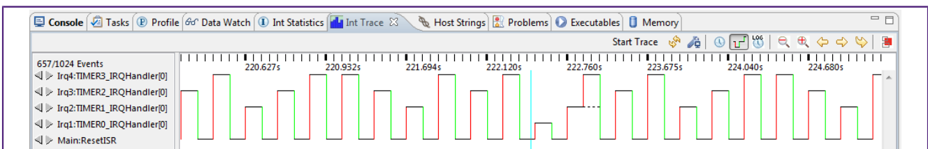
Figure 8.19. Interrupt Trace View
