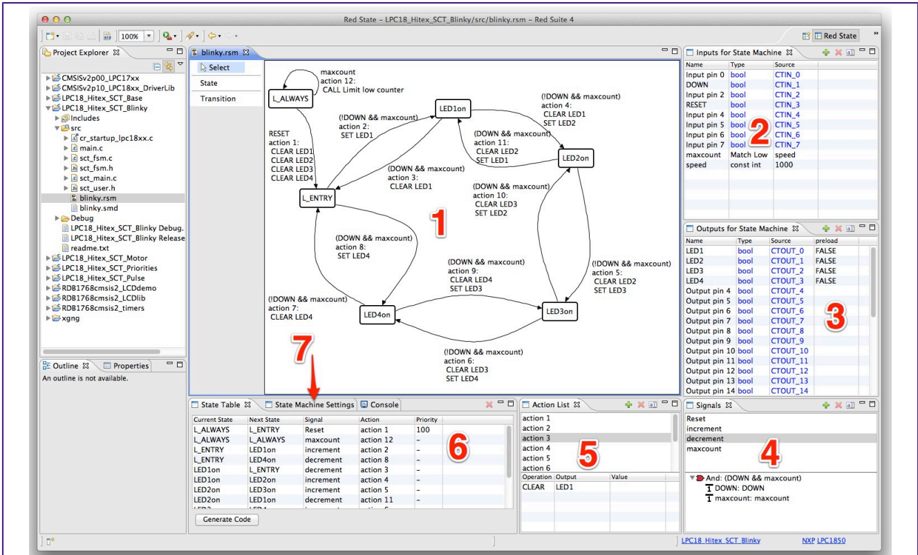
Figure 9.29. The Red State perspective
