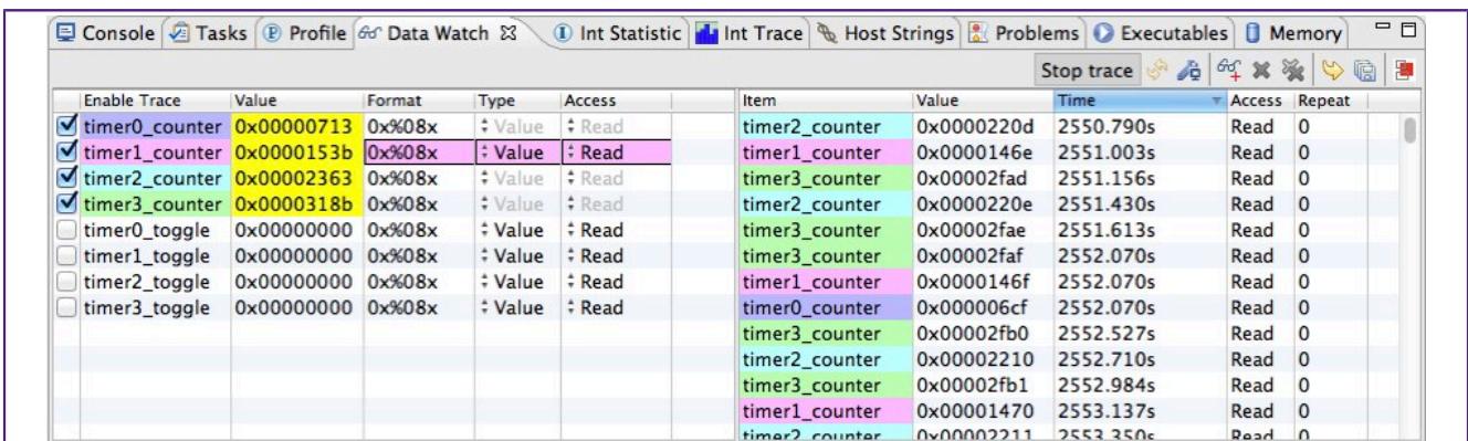
Figure 8.22. Data Watch View
