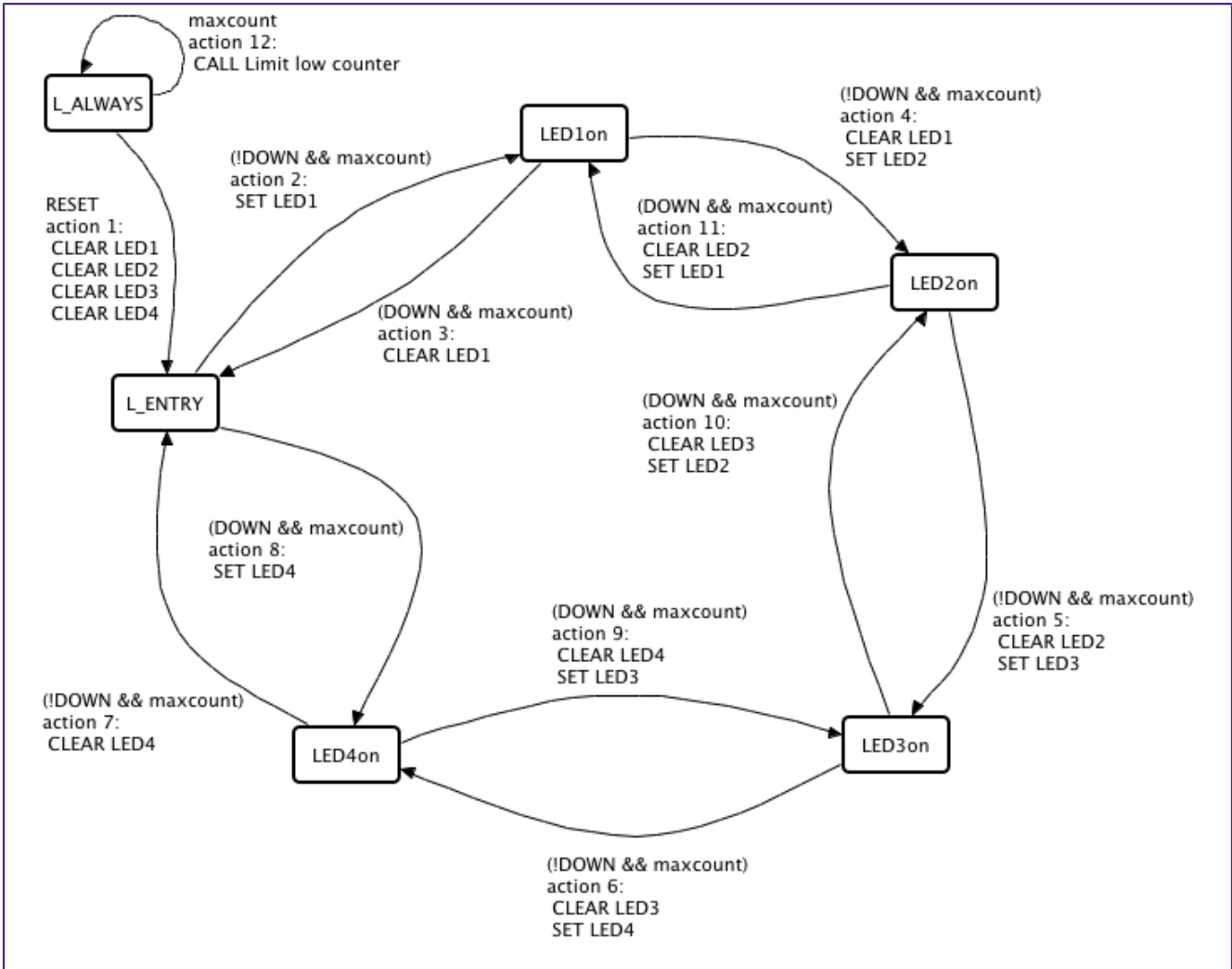
Figure 9.11. The complete state diagram for the SCT blinky example
