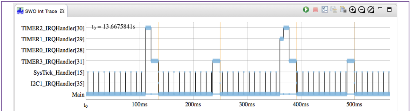
Figure 8.5. SWO Interrupt Statistics View
