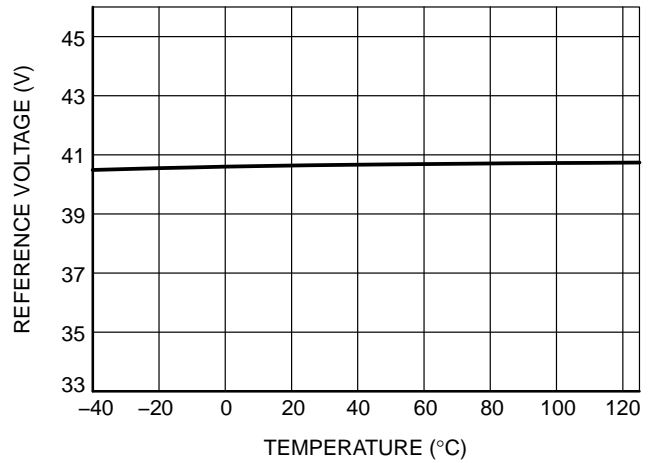
Figure 16. Reference Clamp Voltage
